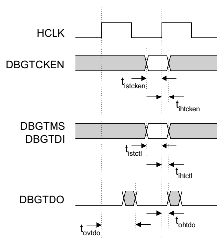
Figure 9-10 Scan timing
